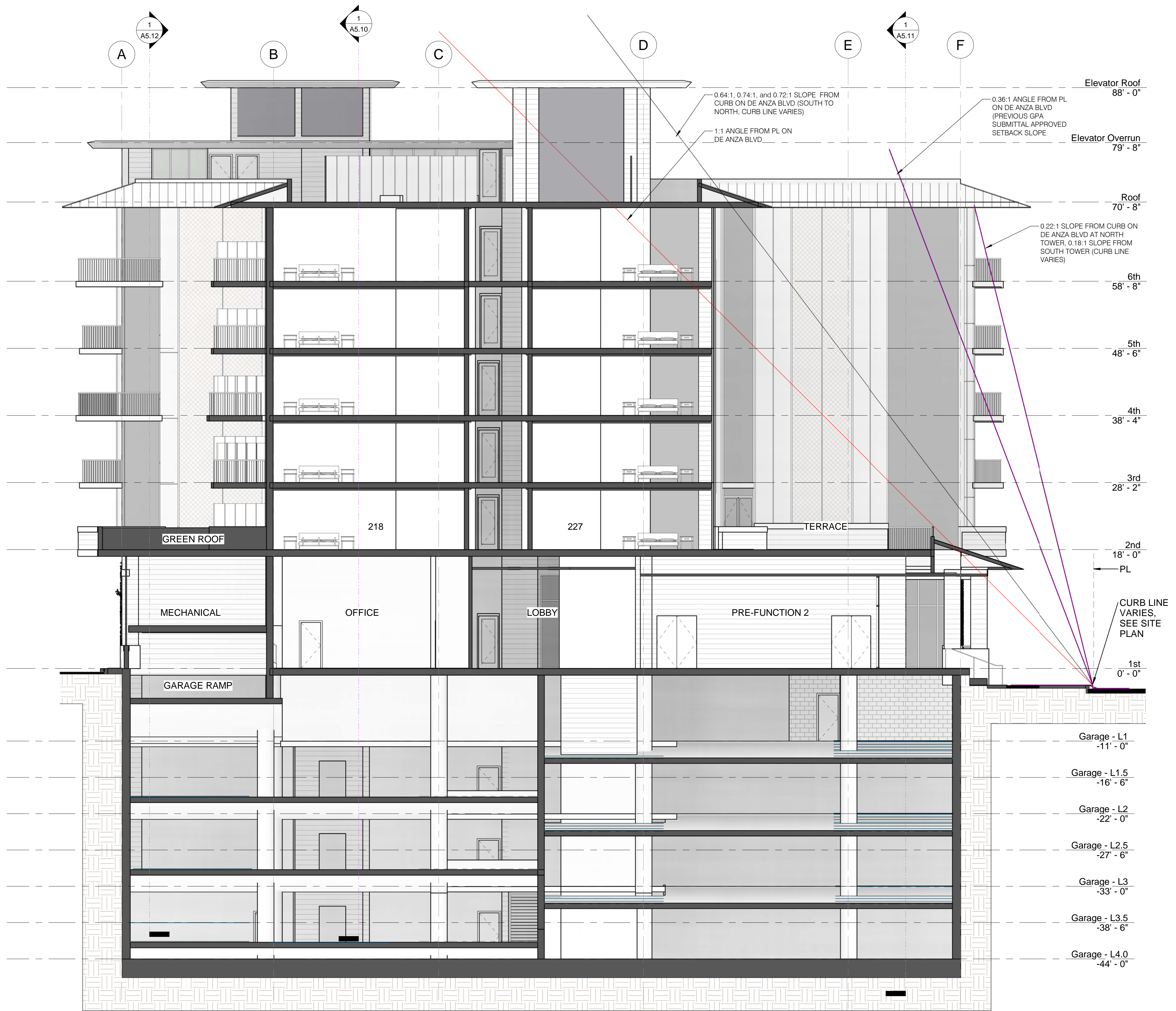
Lateral - through Terrace Looking North 1 1/8" = 1'-0"
