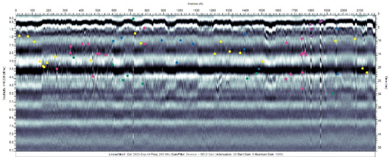
Figure 8 Profile of soils scan showing assumed buried items in colored dots
