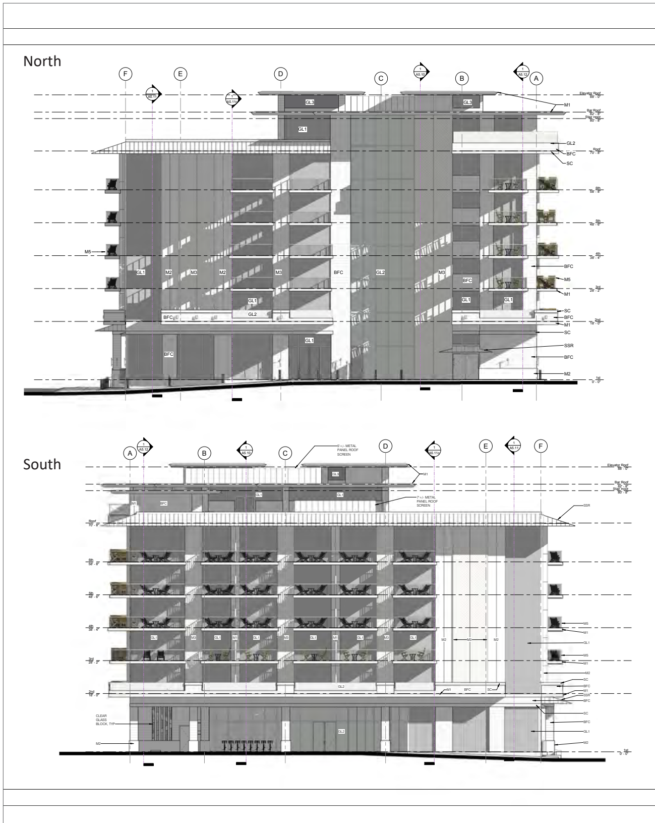
Figure 3-10 North and South Elevations
