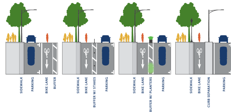
Figure 11: Bicycle Lane Protection Options
